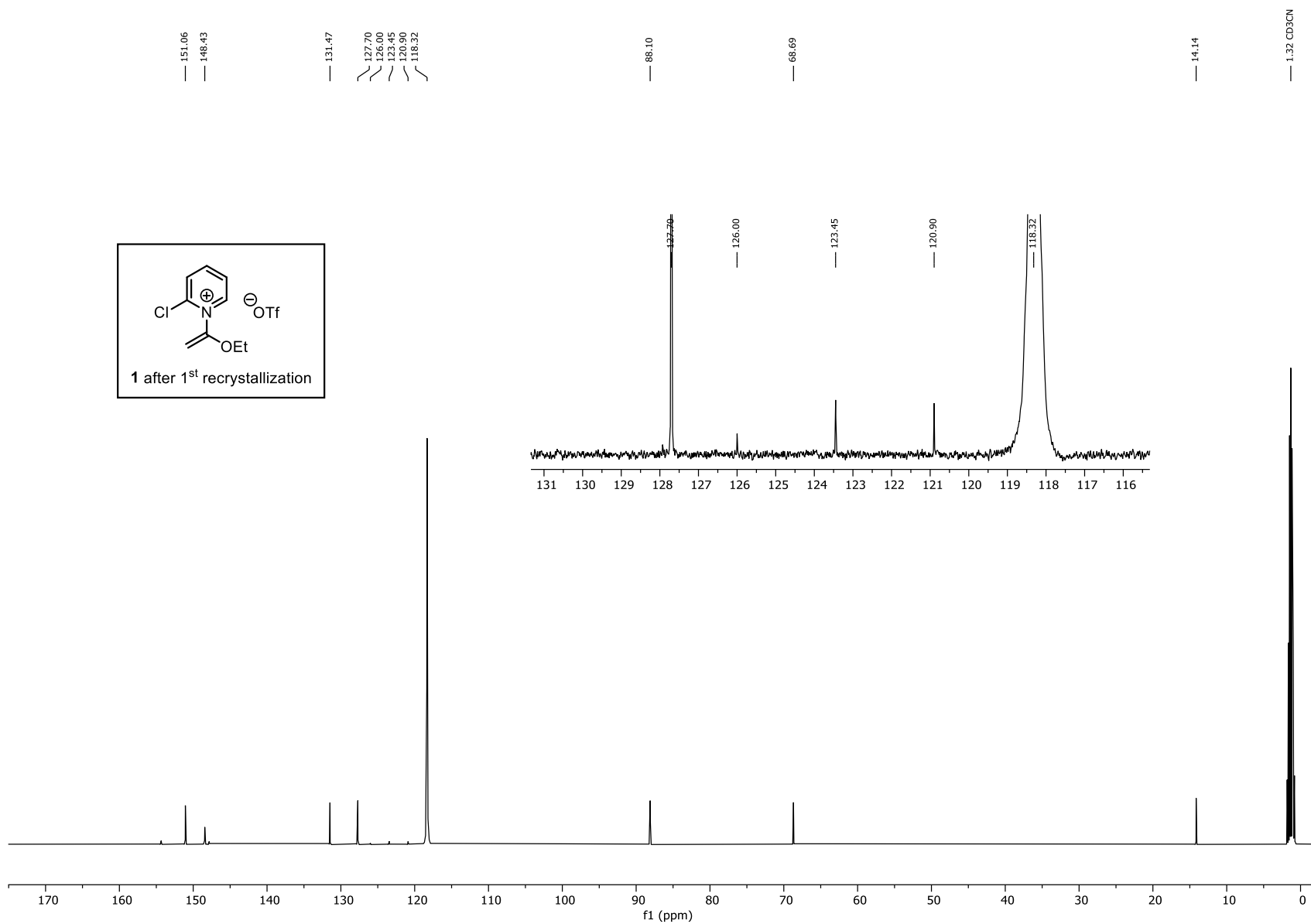
13 C NMR of 1 after 1 recrystallization (126 MHz, CD 3 CN)
